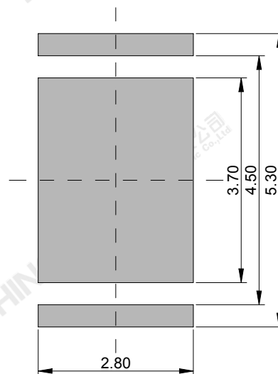
recommended stencil pattern
