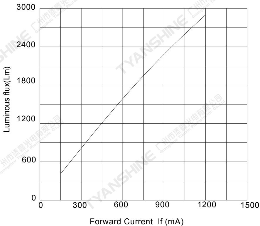
Forward Current VS. Luminous flux
