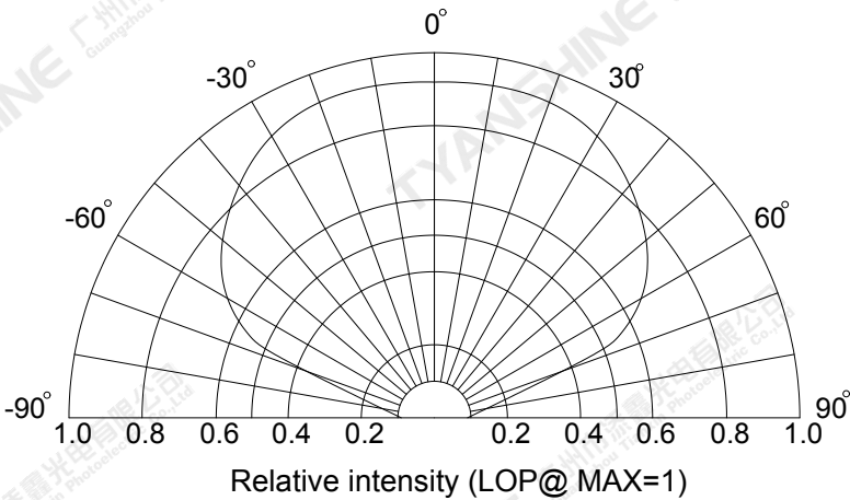
Beam Pattern
