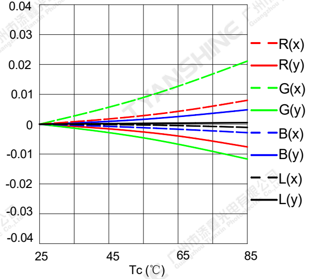
Relative Chromaticity VS. Temperature (IF=0.7A)
