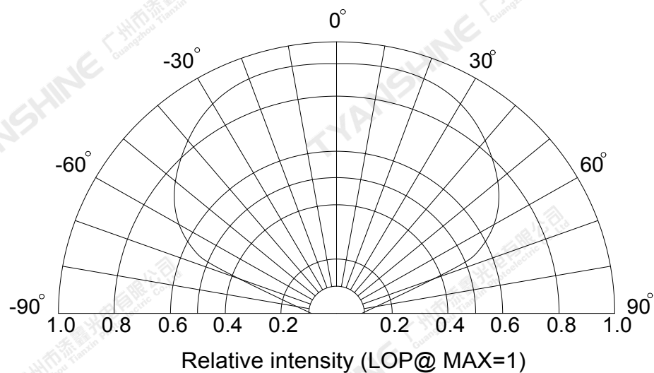
Beam Pattern
